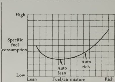
FIGURE 3-3. Specific fuel consumption curve.
